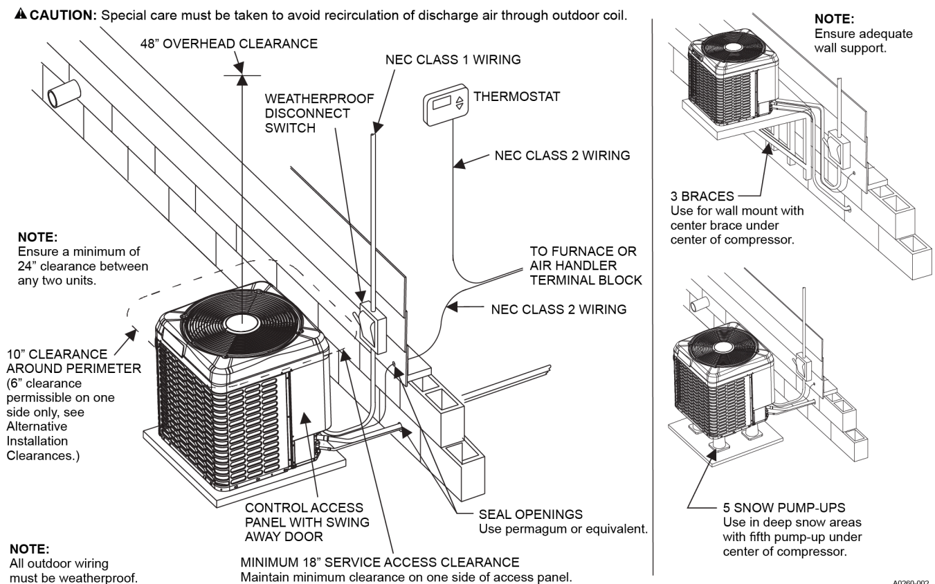
Figure 3: Typical installation
